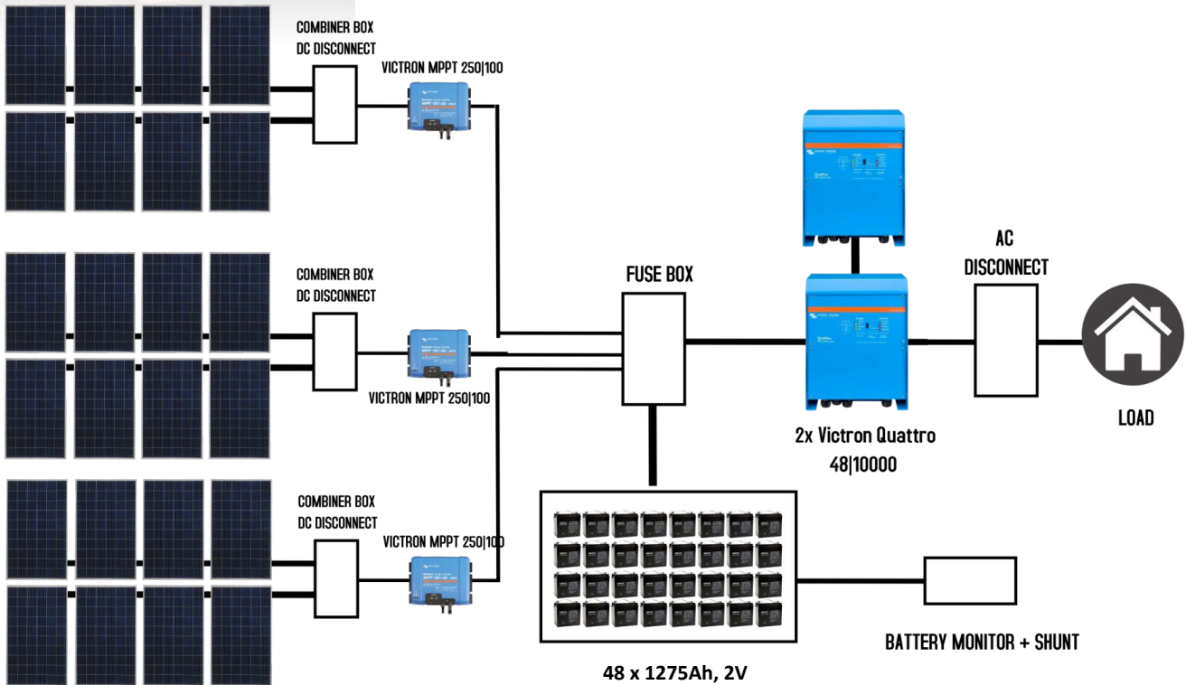
24 x 405W Solar Panel
